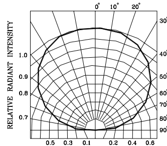
Fig.4 RADIATION DIAGRAM
