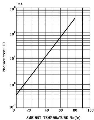
Fig.5 DARK CURRENT mVR=10, Ee=0mw/cm 2 AMBIENT TEMPERATURE
