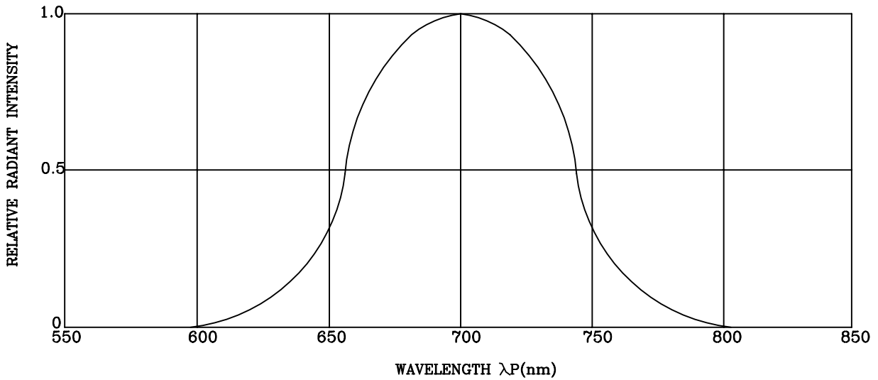
SPECTRAL DISTRIBUTION
