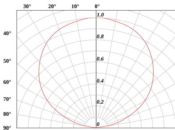
Fig.3 Radiation pattern.
