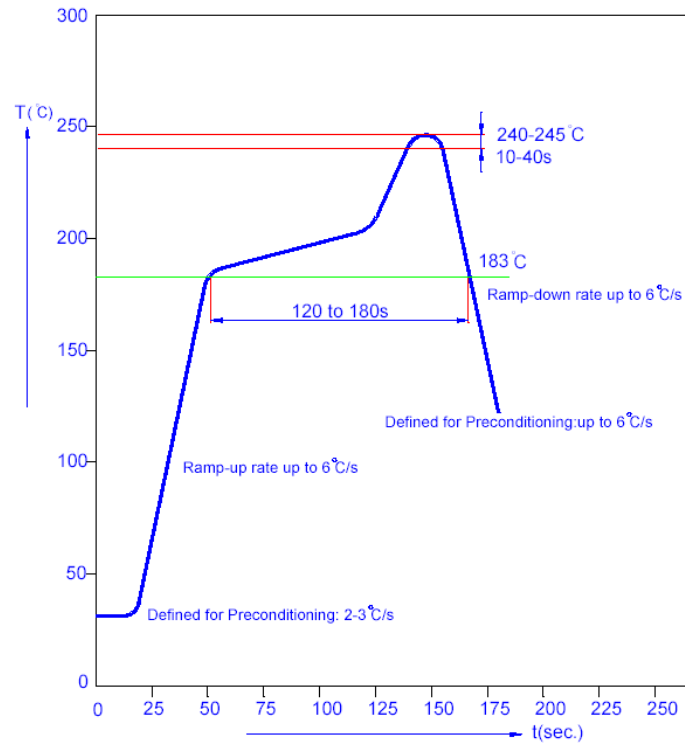
Fig. 5 Recommended IR-reflow Soldering Profile (acc. to IPC 9501)
