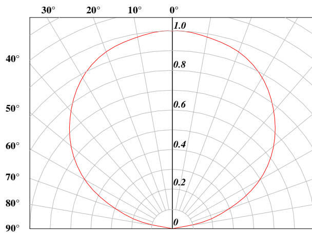
Fig. 3 Radiation pattern.
