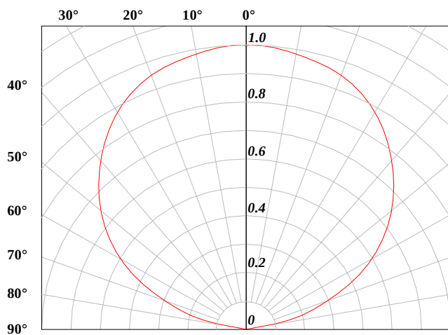
Fig.3 Radiation pattern.
