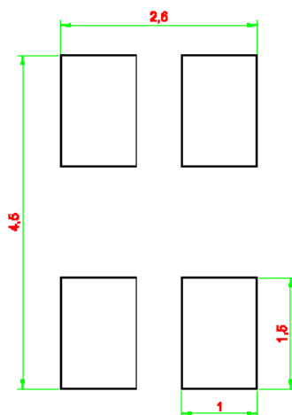
Recommended Solder Pad
