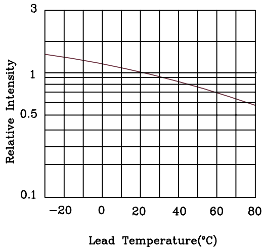
RELATIVE INTENSITY VS. LEAD TEMPERATURE
