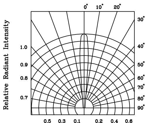
FIG.6 RADIANT DIAGRAM
