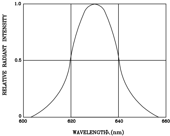
SPECTRAL DISTRIBUTION
