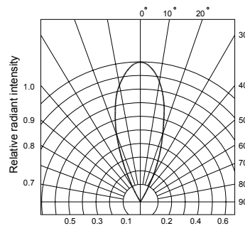
Fig.6 Radiation diagram
