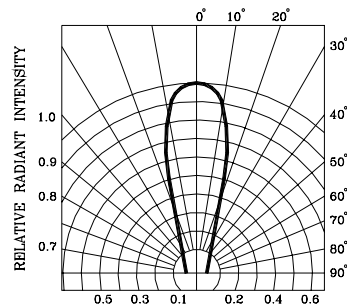
RADIATION DIAGRAM
