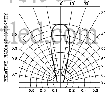
RADIATION DIAGRAM
