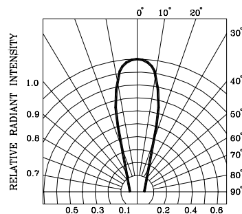
RADIATION DIAGRAM
