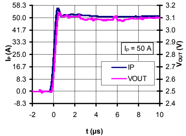
Figure 22: Step response
