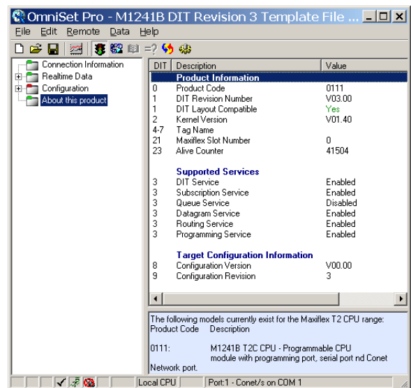
Setting Up a CPU via Omniset Pro
