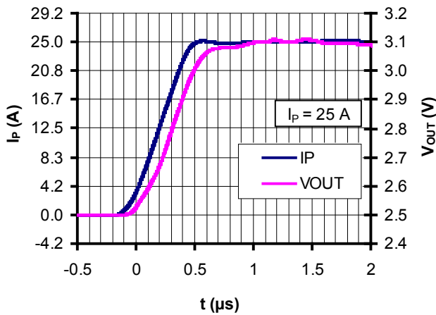
Figure 15: Step response
