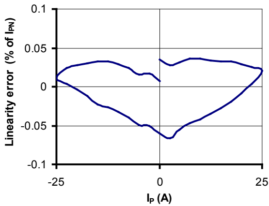
Figure 13: Linearity error
