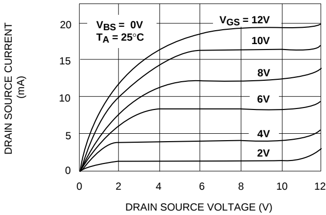
OUTPUT CHARACTERISTICS
