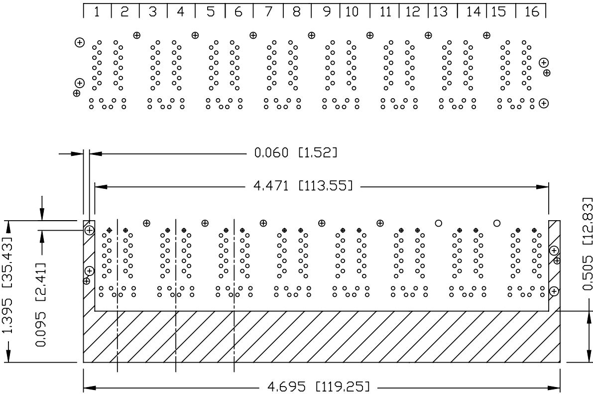
PORT ASSIGNMENT (COMPONENT SIDE VIEW)
