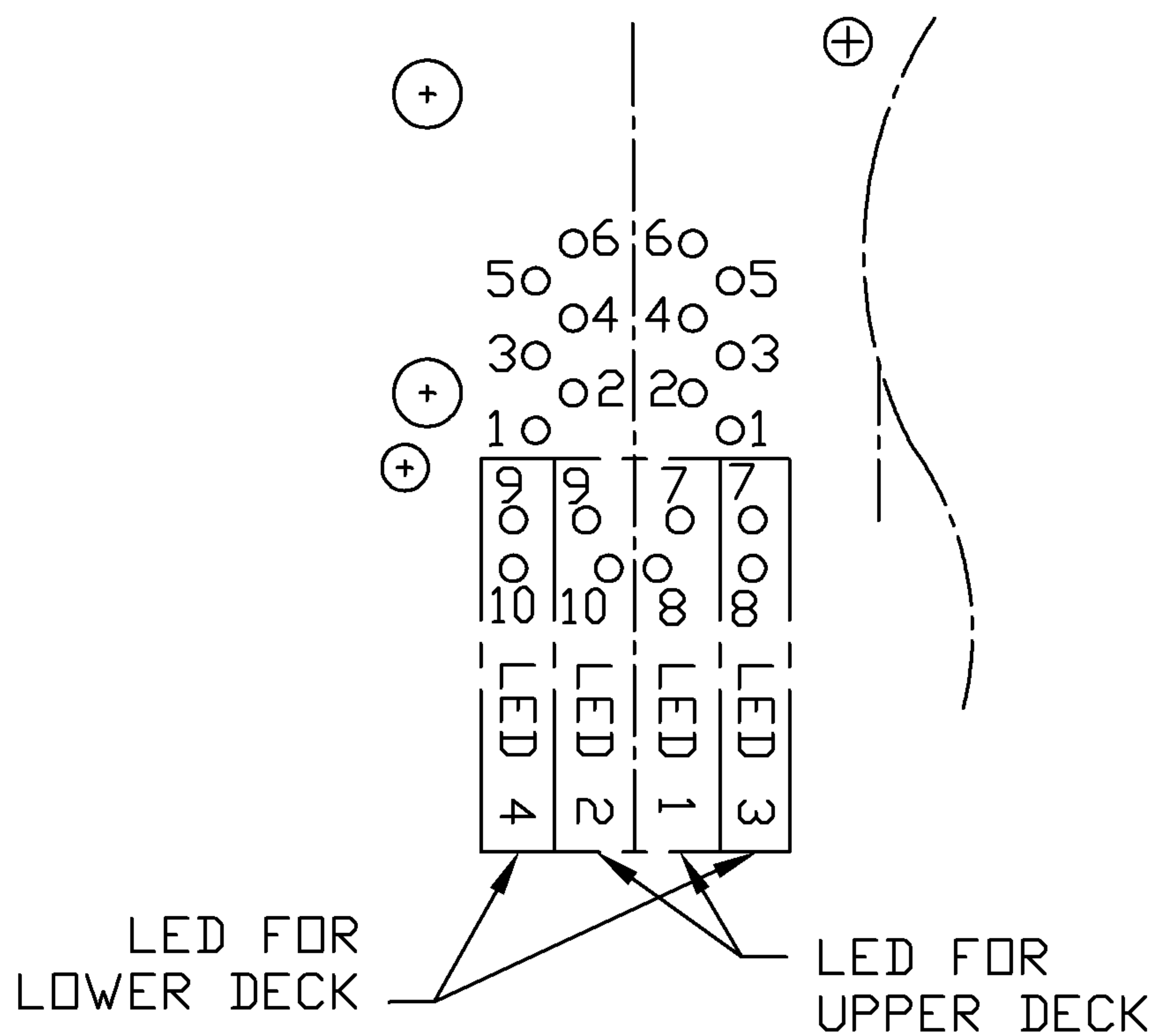
PIN-OUT INFORMATION (COMPONENT SIDE VIEW)
