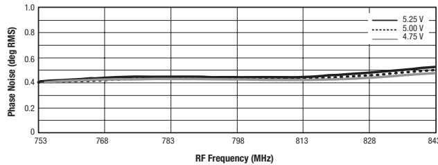
Figure 13. Integrated Phase Noise vs Frequency and Supply Voltage
