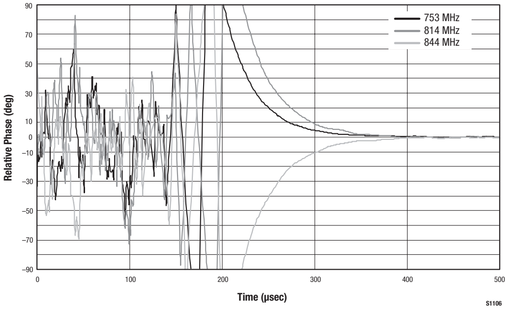
Figure 9. Phase Settling Time Measurements
