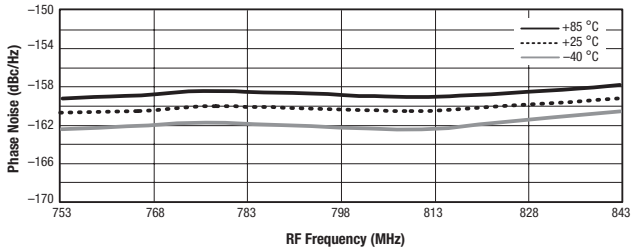
Figure 24. Phase Noise @ 1800 kHz Offset vs Frequency and Temperature
