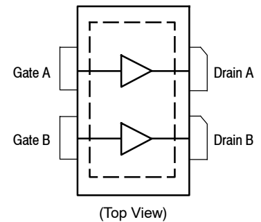
Figure 1. Pin Connections
