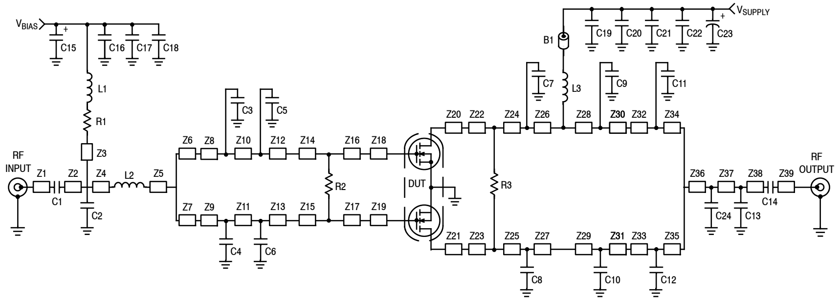
Figure 11. AFT05MP075NR1(GNR1) UHF Broadband Reference Circuit Schematic — 450-520 MHz
