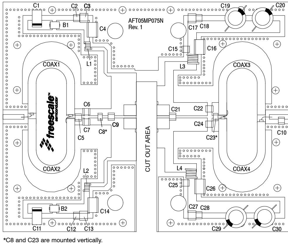
Figure 5. AFT05MP075NR1(GNR1) Narrowband Test Circuit Component Layout — 520 MHz
