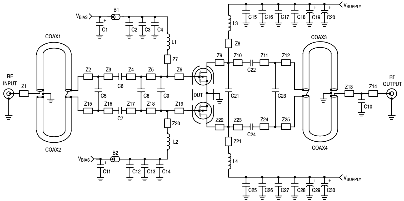
Figure 6. AFT05MP075NR1(GNR1) Narrowband Test Circuit Schematic — 520 MHz
