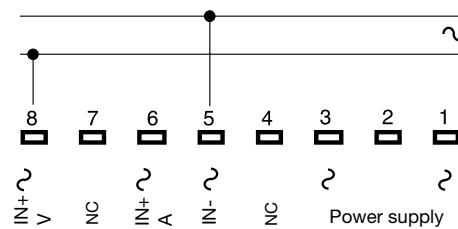
Voltage measurements - direct
