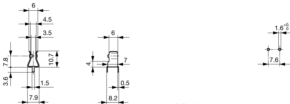
Drilling diagram
