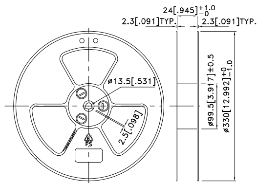
Reel Dimension
