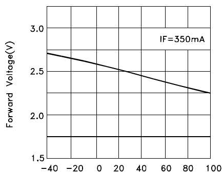
Ambient Temperature TA(°C) FORWARD VOLTAGE VS. AMBIENT TEMPERATURE
