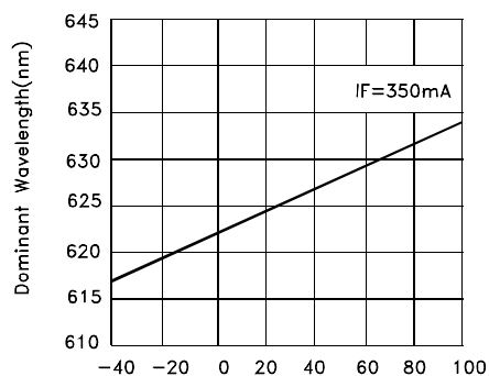
Ambient Temperature TA(°C) DOMINANT WAVELENGTH VS. AMBIENT TEMPERATURE
