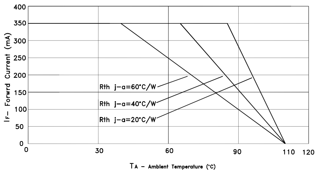
Current Derating Curves
