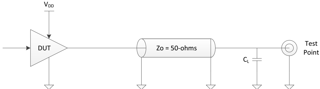
Figure 3: Test Circuit Load used for AC timing
