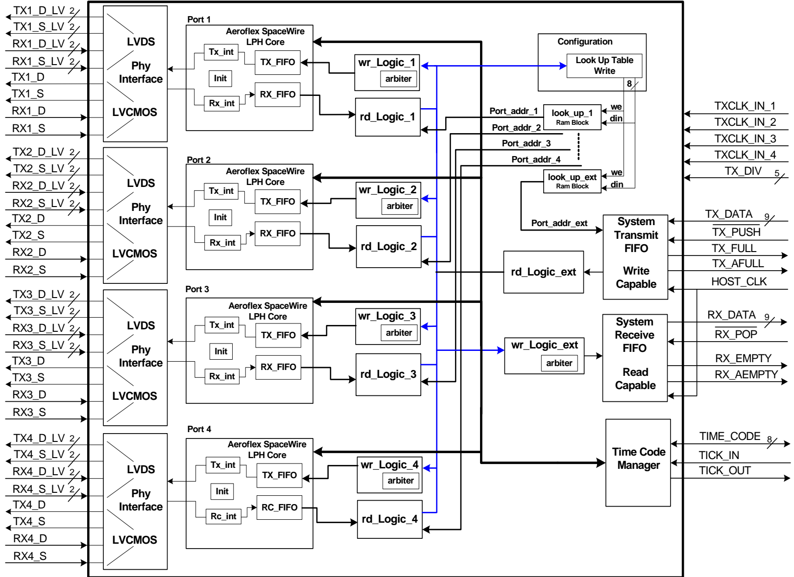
Figure 1. UT200SpW4RTR SpaceWire 4-Port Router Block Diagram
