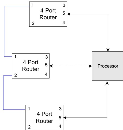
Figure 15. 8-Port Extended Configuration Using uP
