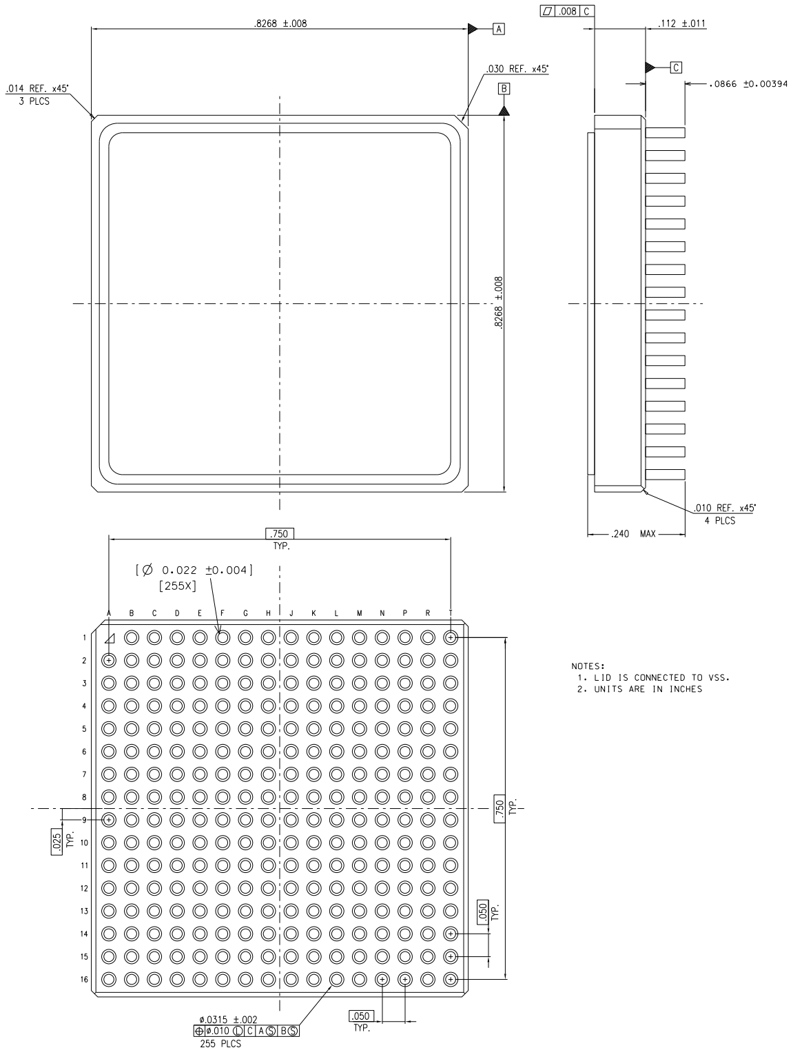
Figure 40. 255-CCGA
