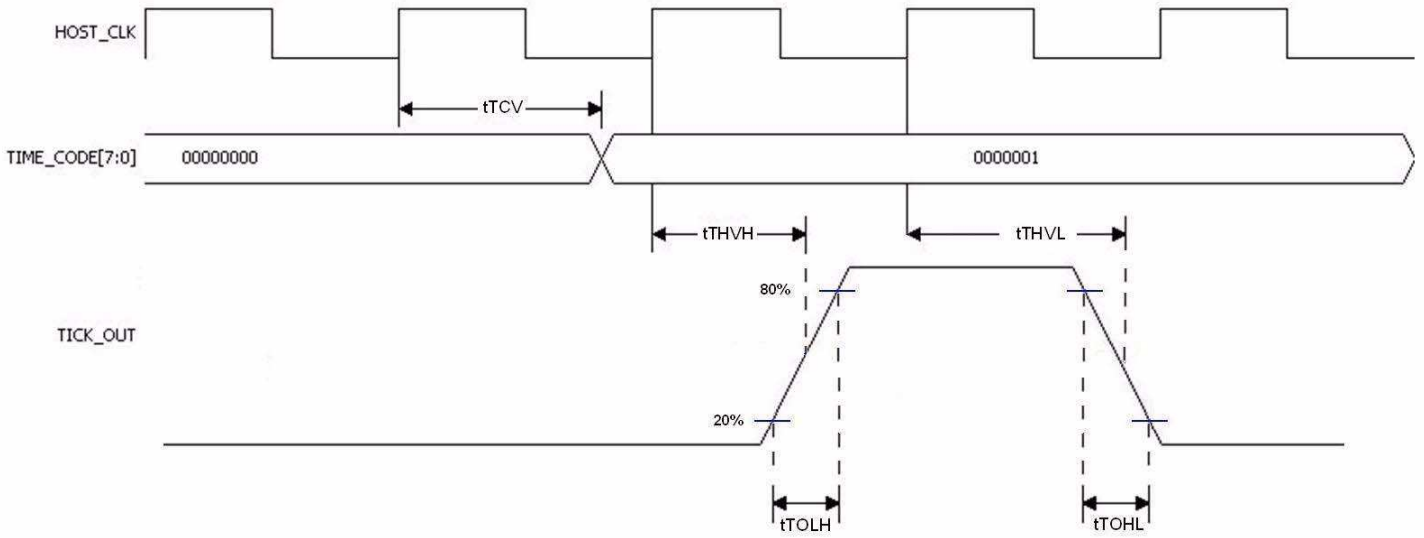
Figure 31. TICK_OUT Interface
