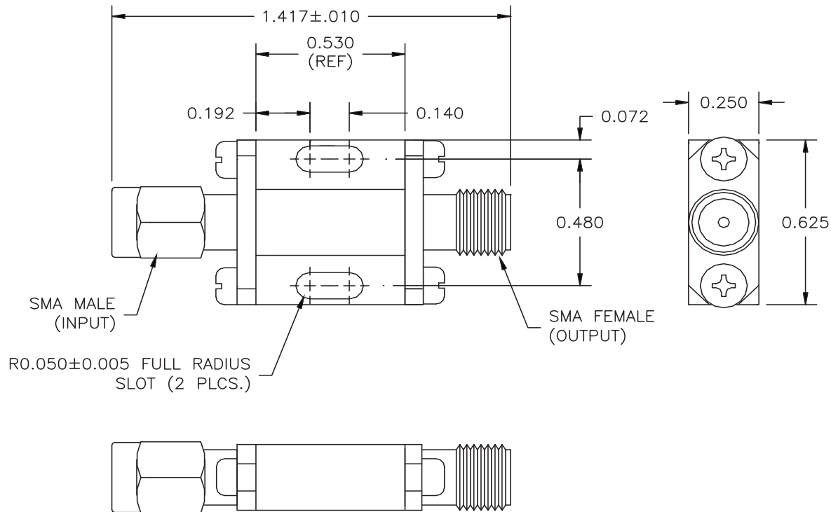
STANDARD CASE STYLE C36 (Optional Case Styles – C37, M61)
