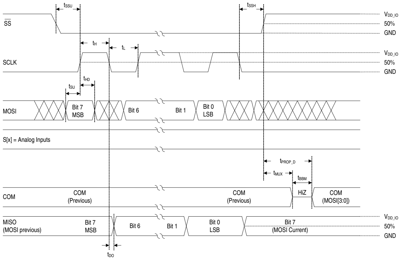
Figure 5. UT16MX117 Timing Diagram
