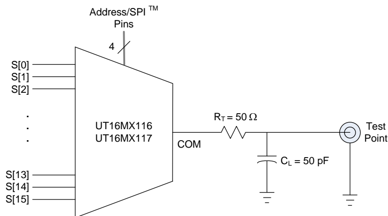
Figure 10. UT16MX116/117 Test Circuit
