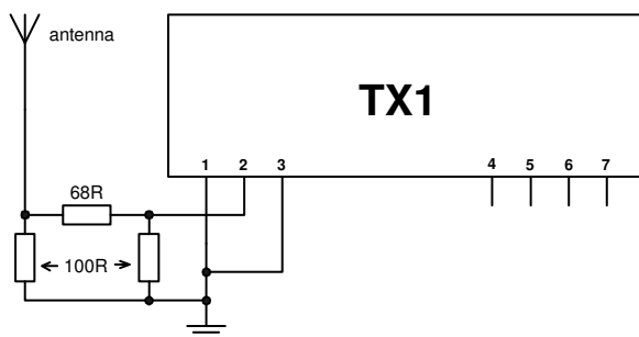
schematic diagram
