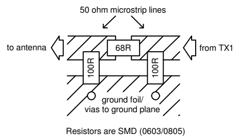
physical arrangement
