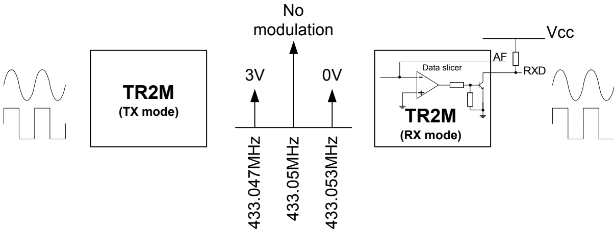
Figure 9: Data polarity change from TR2M (in transmit mode) to TR2M (in receive mode)
