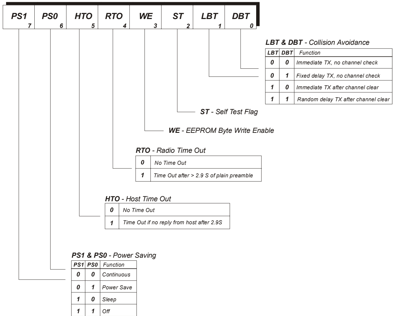
figure 11: Switches
