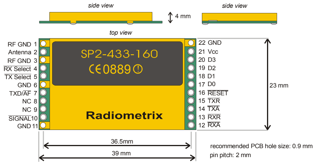
figure 3: Pin out and physical dimension
