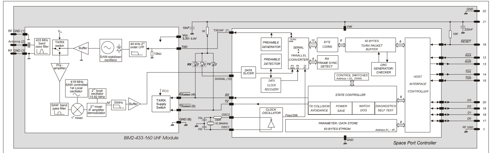
figure 2: SP2-433-160 block diagram
