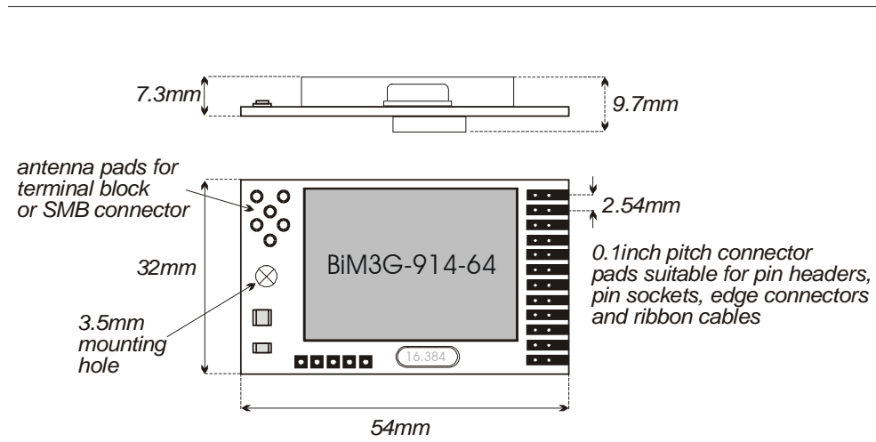
figure 3: physical dimensions
