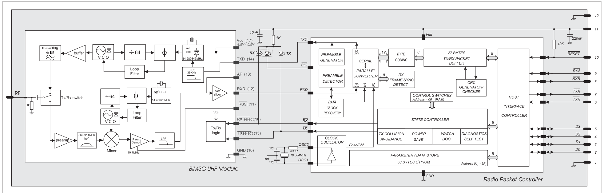
figure 2: RPC3G block diagram
