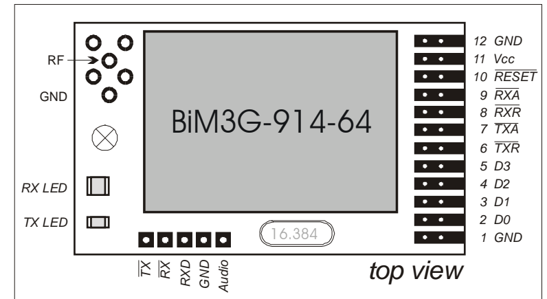
figure 4: RPC3G's pinout
