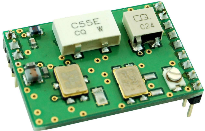
Figure 1: CVR1-169.4125-10 receiver (top)
