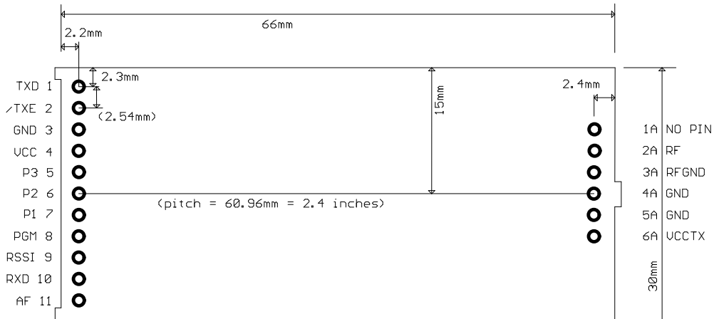
Figure 3: SHX1 footprint (Top) view
