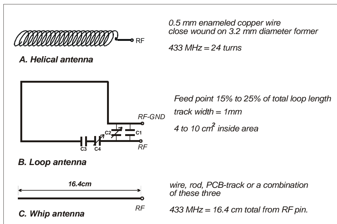
Fig.6: Antenna configuration
