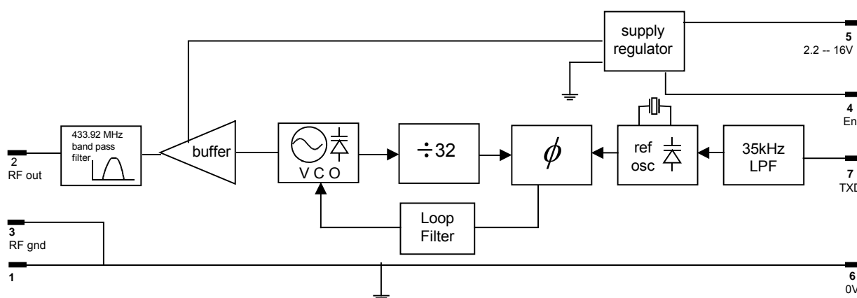
Fig. 2: TX2A block diagram
