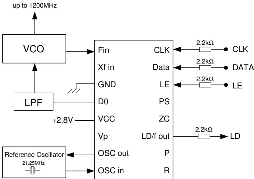
Figure 4: PLL IC Control
