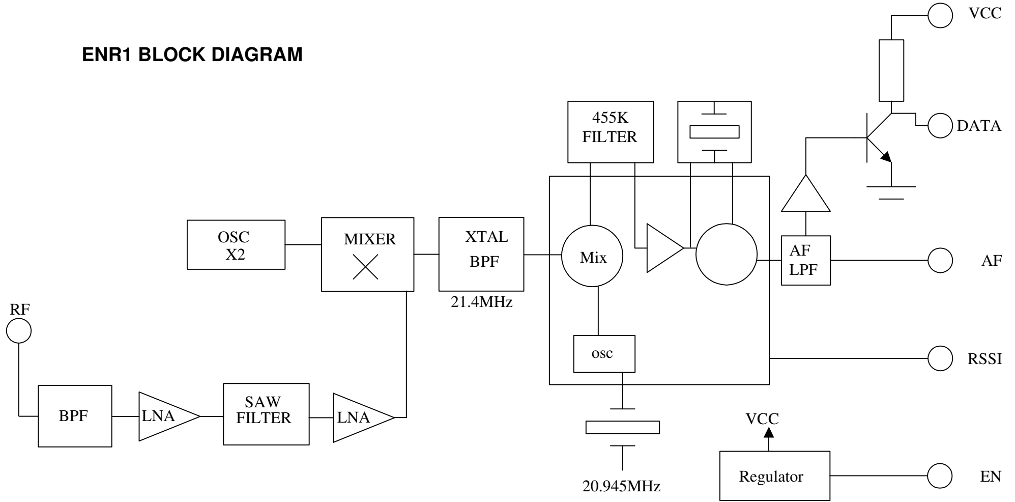
Figure 4: ENR1 block diagram
