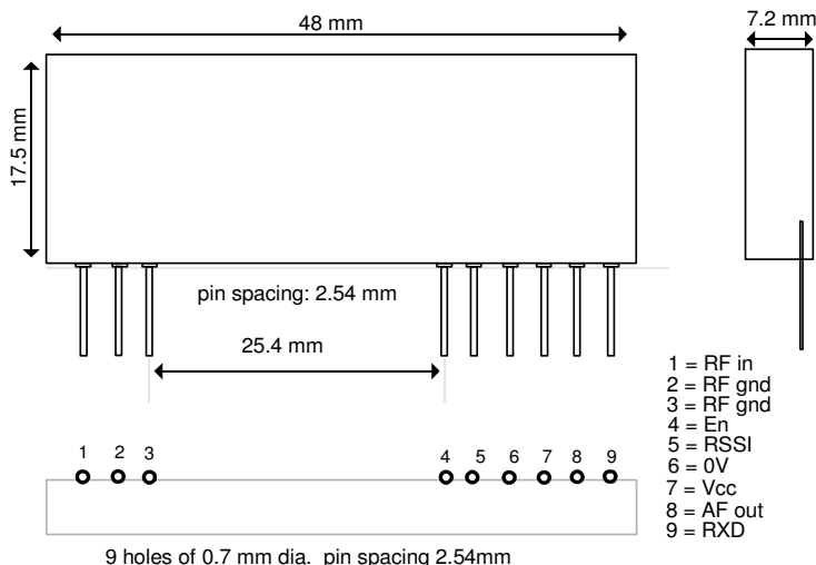
Figure 5: ENR1 pin-out and dimension
