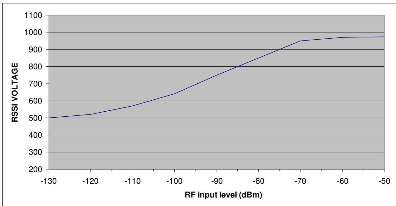
Figure 3: Typical RSSI response
