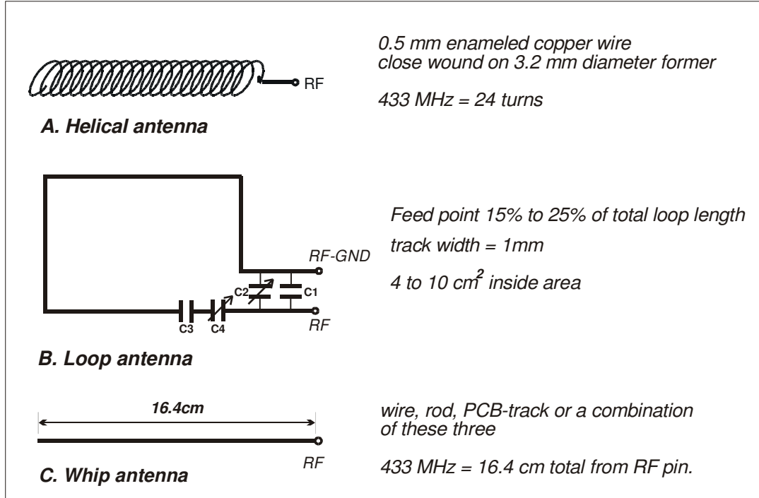
Figure 10: Antenna types
