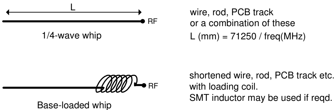
Fig. 5: Antenna configurations
