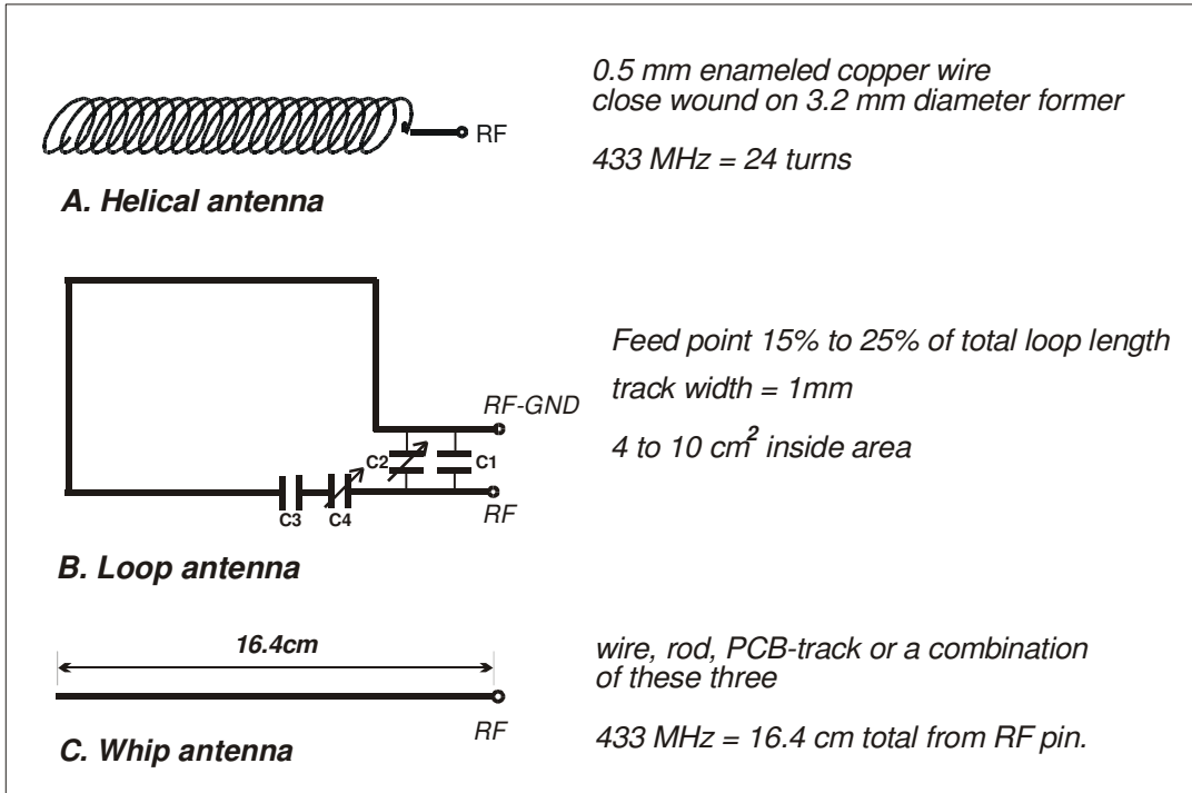
Figure 6: Antenna configuration
