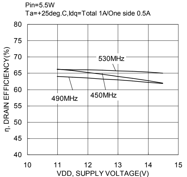
Drain Efficiency versus Supply Voltage
