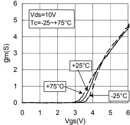
Vgs-gm CHARACTERISTICS
