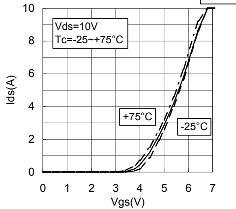
Vgs-Ids CHARACTERISTICS 2
