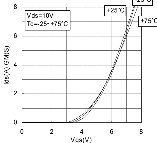
Vgs-Ids CHARACTERISTICS 2
