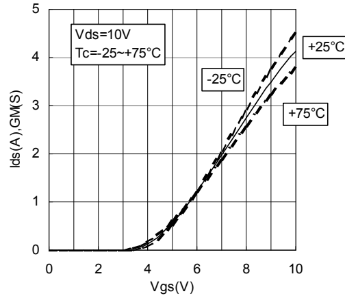
Vgs-Ids CHARACTERISTICS 2
