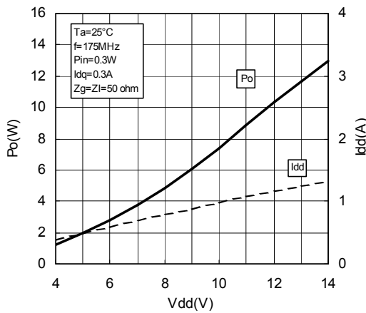
Vdd-Po CHARACTERISTICS
