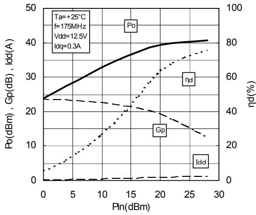
Pin-Po CHARACTERISTICS
