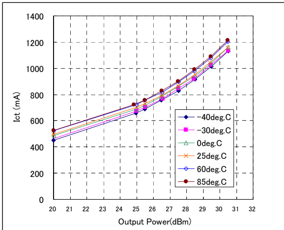
Operating Current vs. Output Power
