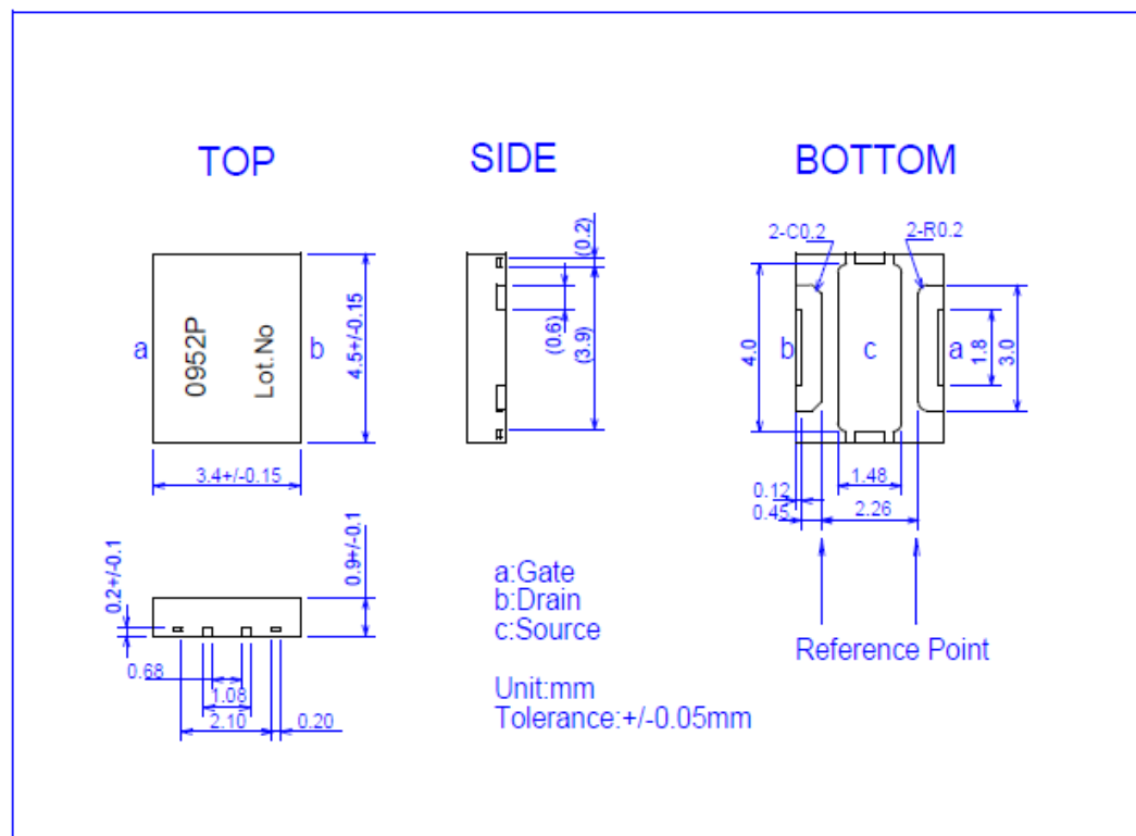
Fig1. OUTLINE DRAWING
