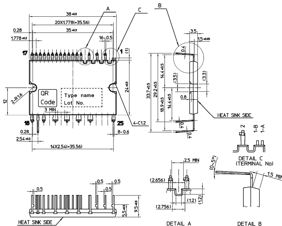
Fig. 10 Package Outlines
