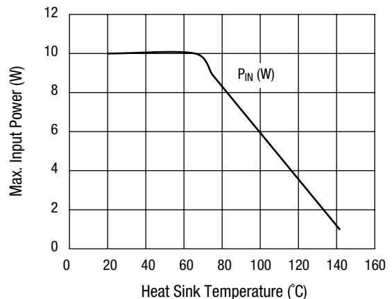
Temperature Derating Curve (0, +10)
